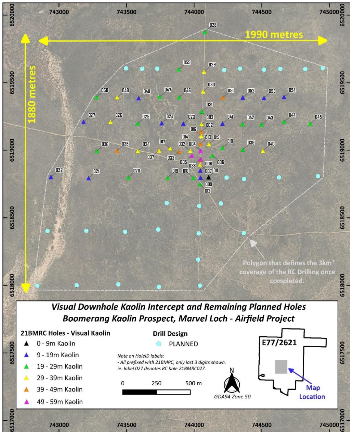
Figure 2. Map showing location of completed RC holes, coloured by depth of vertical kaolin intercept (as determined by geologist on rig), and location of remaining planned drillholes
