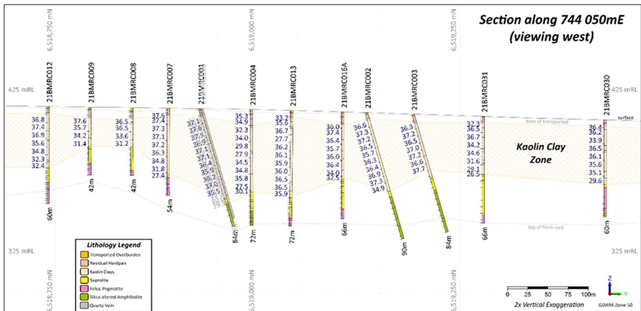
Figure 1: Cross section through 744,050mE (viewing west) showing % Al 2 O 3 within the -45µm size fraction for the Kaolin clay zone, and interpreted base of transported and top of fresh rock boundaries. Location of cross section provided in Figure 3. Note: Results for 21BMRC038 (drilled as a duplicate hole of 21BMRC001) have been greyed out for ease of reading.
